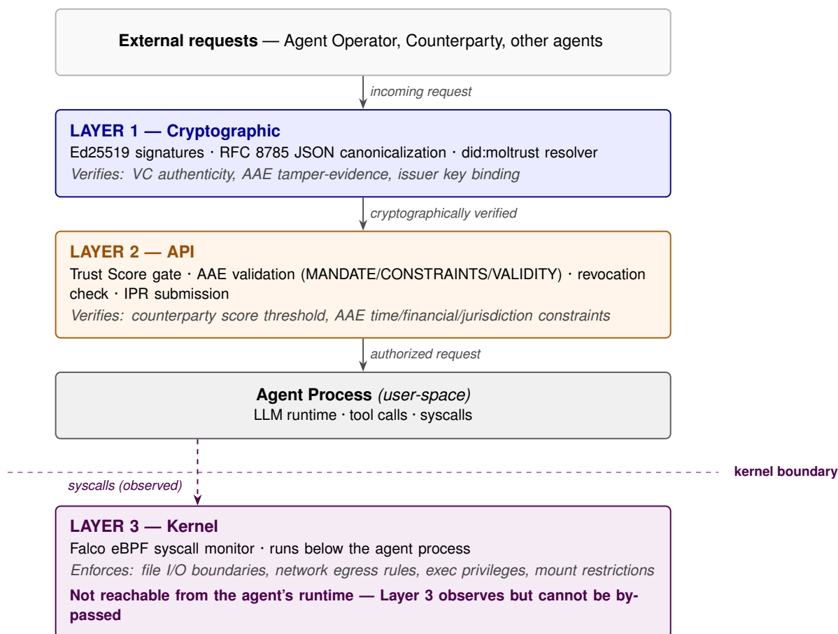
Figure 3: Three-layer enforcement architecture. External requests are verified cryptographically (Layer 1), then validated against the AAE policy and trust score gates (Layer 2), before reaching the Agent Process in user-space. Independently of the agent’s runtime, Falco eBPF (Layer 3) observes syscalls from below the kernel boundary and records violations as permanent trust events. Layer 3 is unby-passable from the agent’s own runtime — enforcement sits below the agent process, not above it.
