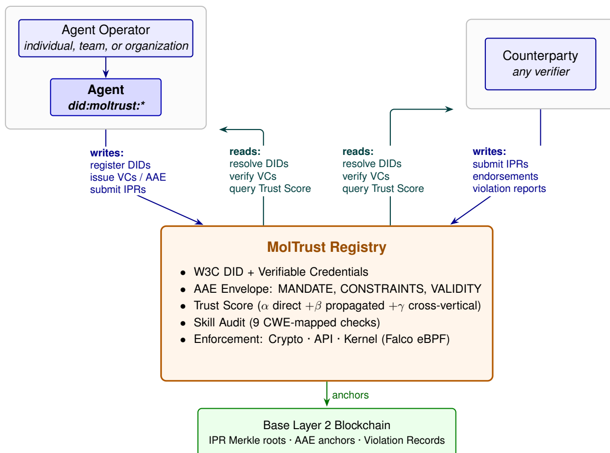
Figure 1: MolTrust Protocol architecture. The Registry mediates between Agent Operators (individuals, teams, or organizations deploying autonomous agents) and Counterparties (any verifier — another agent, an enterprise system, or a regulatory auditor). Both sides write evidence to the Registry (DIDs, VCs, AAE envelopes, Interaction Proof Records, endorsements, violation reports) and read attestations from it (DID resolution, VC verification, Trust Score queries). The Registry anchors cryptographic commitments on Base Layer 2 for independent verifiability. No single platform, vendor, or jurisdiction is in the trust path.
