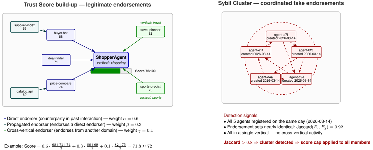
Figure 4: Trust Score build-up and Sybil Cluster detection. Left: a legitimate agent (ShopperAgent, vertical shopping) accumulates a Trust Score of 72/100 through weighted endorsements from direct counterparties ( \alpha = 0.6 ), propagated endorsers ( \beta = 0.3 ), and cross-vertical endorsers from other domains ( \gamma = 0.1 ). Right: a coordinated ring of five agents (agent-a7f through agent-e1f), all registered on the same day with near-identical endorsement sets ( Jaccard = 0.92 ) and no cross-vertical activity, is automatically detected and score-capped. The Jaccard threshold ( > 0.8 ) and the mandatory cross-vertical diversity (minimum three verticals) are the two structural constraints that make coordinated fake-endorsement campaigns economically ineffective.
